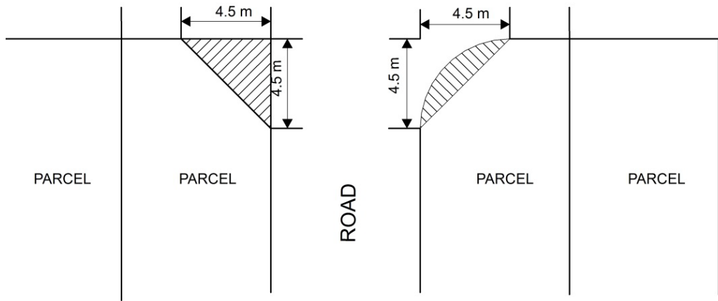
Figure 6 – Sight Triangle
