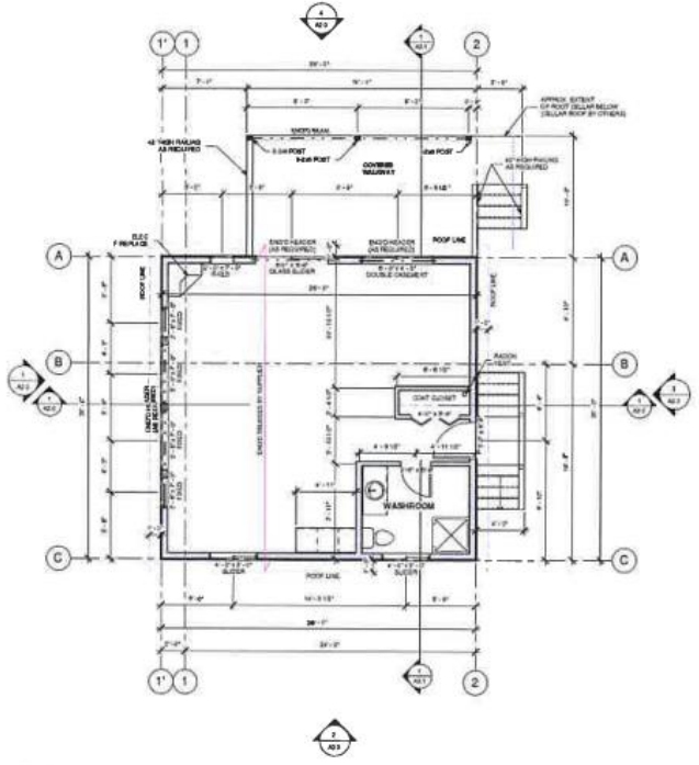
3 2nd Floor Plan 1/4" = 1'-0"
