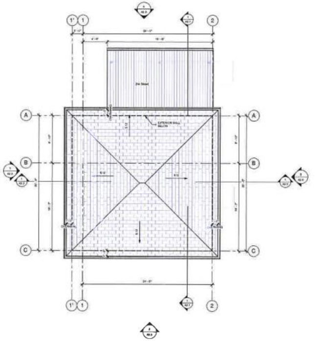
4 Roof Plan 1/4" = 1'-0"
