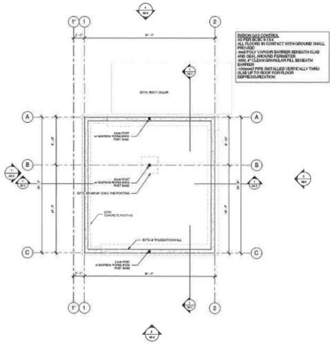
1 Basement Floor 1/4" = 1'-0"
