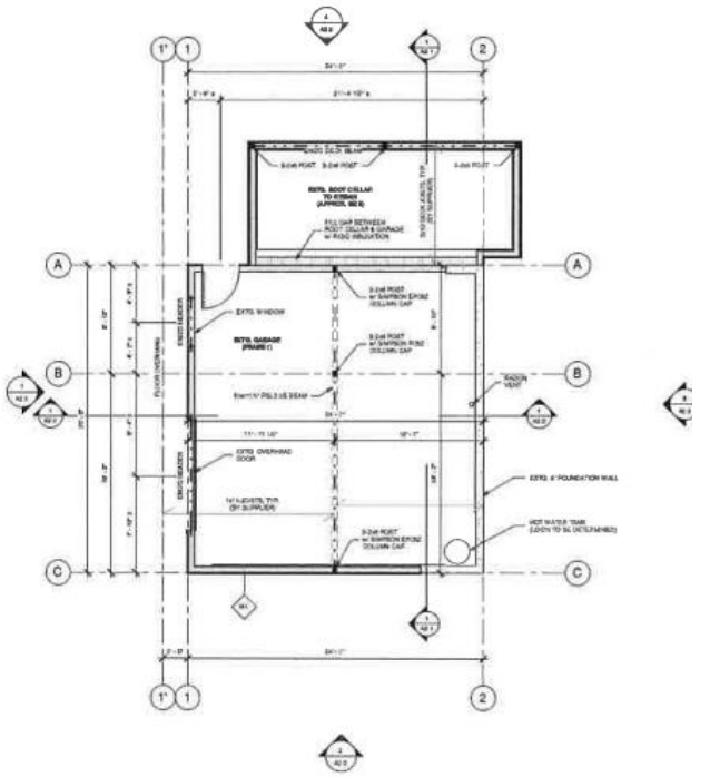
2 1st Floor Plan 1/4" = 1'-0"
