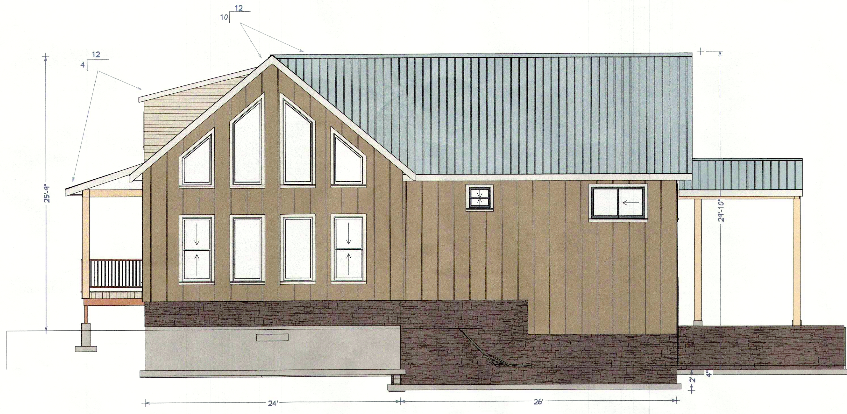
Exterior Elevation Left (new construction)
