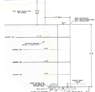
7 12.5' HEIGHT RTG WALL (SLOPED BACKFILL) C0.2 SCALE: 3/8" = 1' 0"
