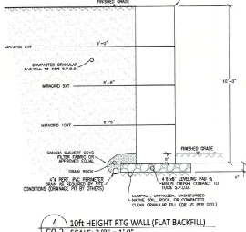
4 10' HEIGHT RTG WALL (FLAT BACKFILL) C0.2 SCALE: 3/8" = 1' 0"
