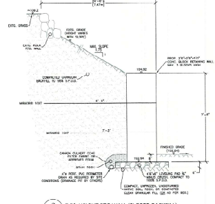
3 7.5' HEIGHT RTG WALL (SLOPED BACKFILL) C0.2 SCALE: 3/8" = 1' 0"
