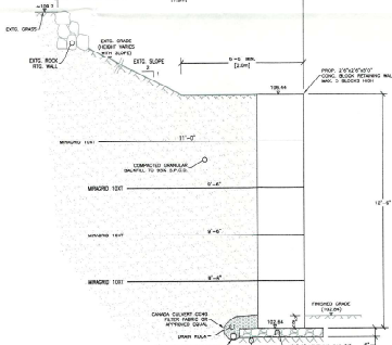
6 12.5' HEIGHT RTG WALL (SLOPED BACKFILL) C0.2 SCALE: 3/8" = 1' 0"
