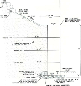
5 10' HEIGHT RTG WALL (SLOPED BACKFILL) C0.2 SCALE: 3/8" = 1' 0"
