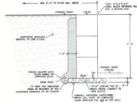
2 UP TO 7.5' HEIGHT RTG WALL (FLAT BACKFILL) C0.2 SCALE: 3/8" = 1' 0"
