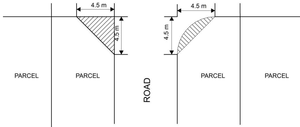
Figure 5 – Sight Triangle
