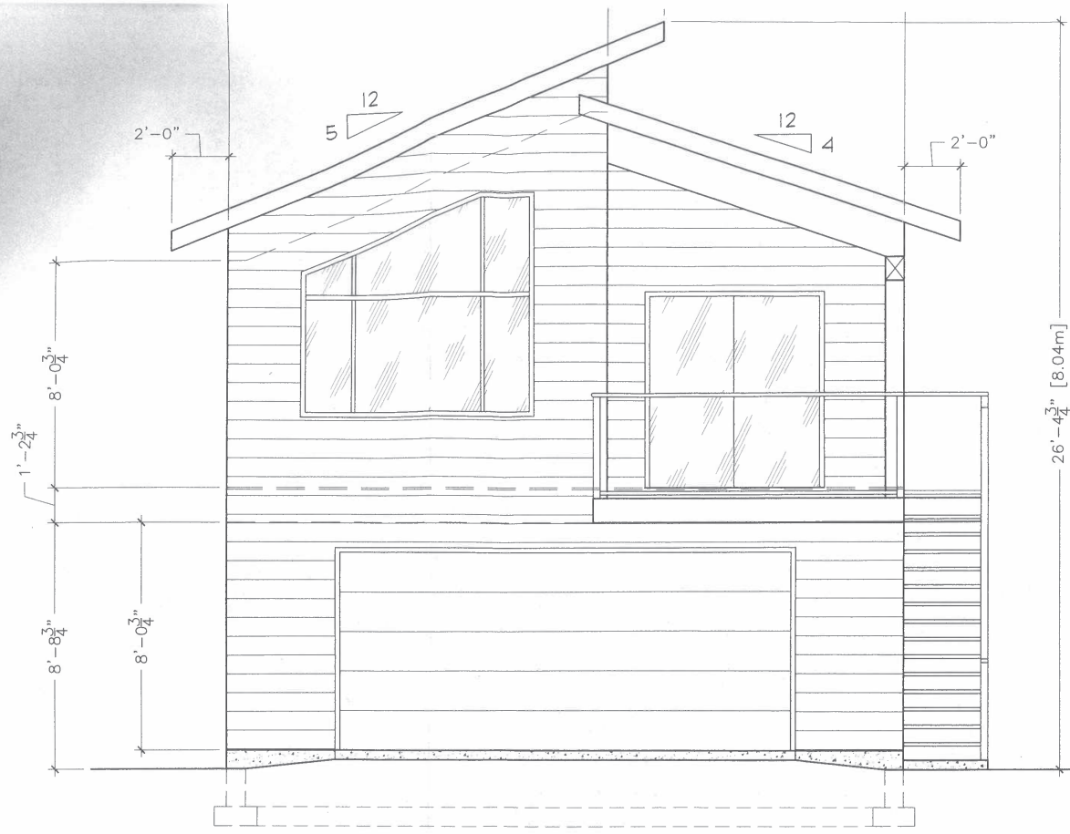
SOUTHEAST ELEVATION
