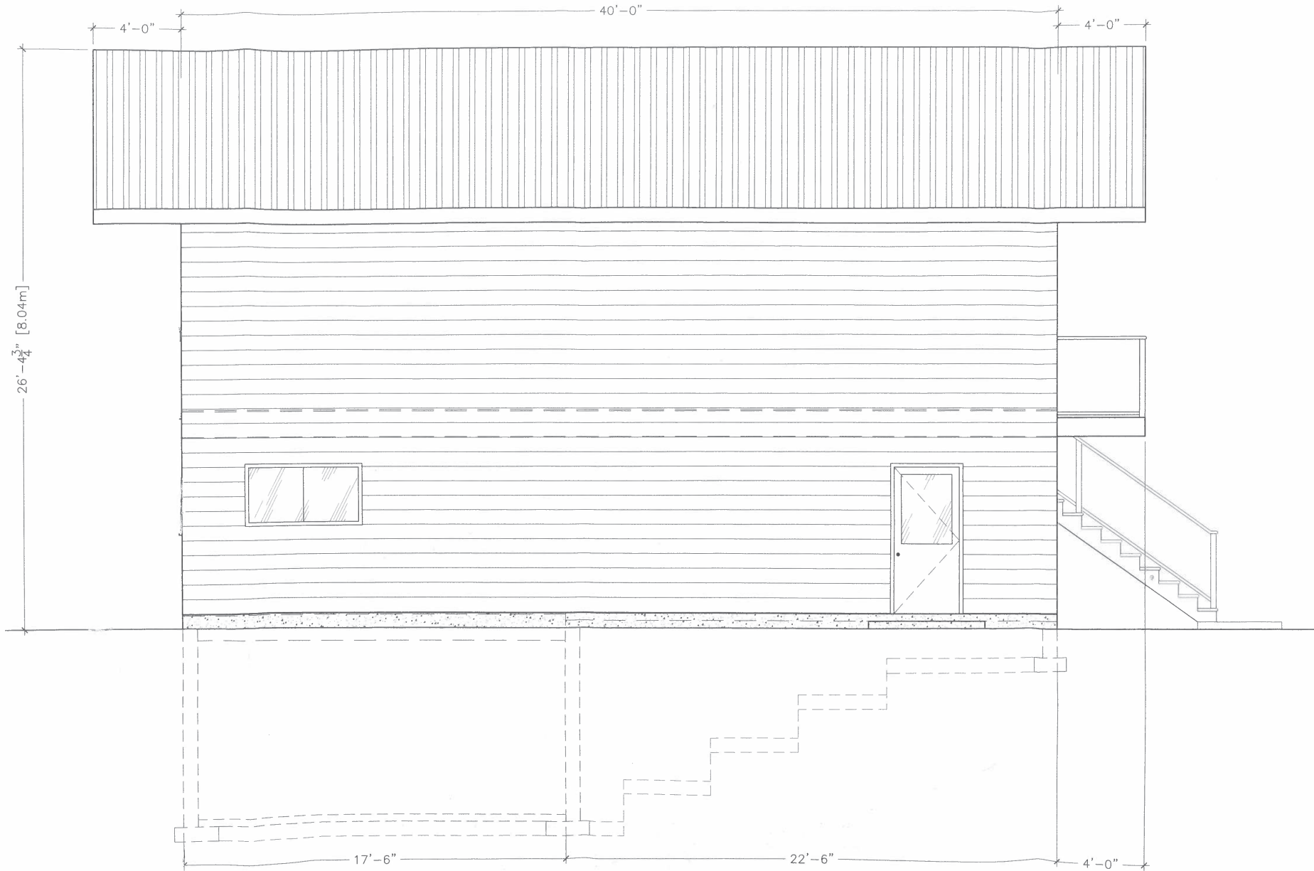
SOUTHWEST ELEVATION
