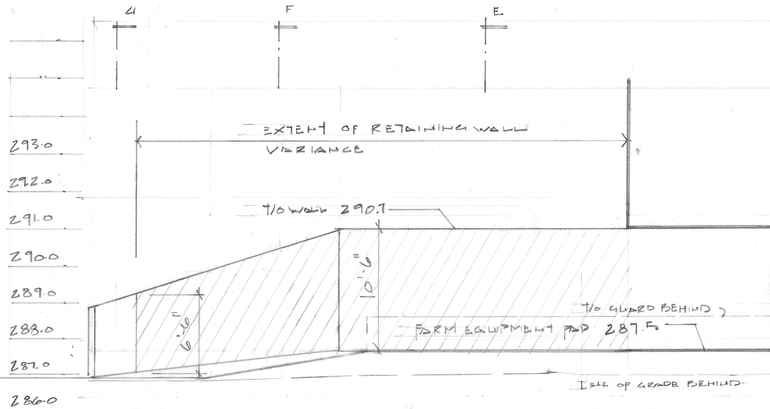
FARM EQUIPMENT PAD (EAST) RETAINING WALL
